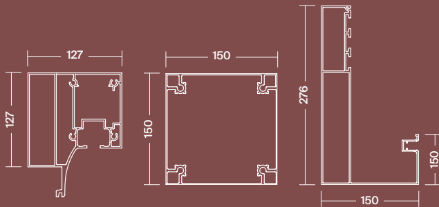
Runner Glissière
